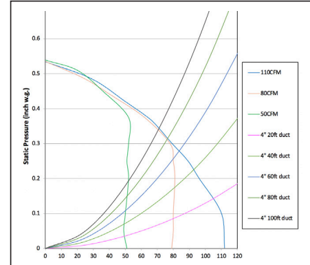
FV-0511VFL1 - 4" Duct
