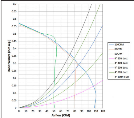
FV-0511VF1 - 4" Duct
