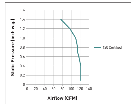
FV-12VE1S Net Supply
