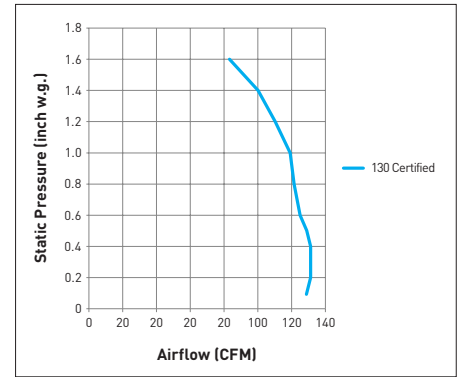
FV-15VE1S Net Supply
