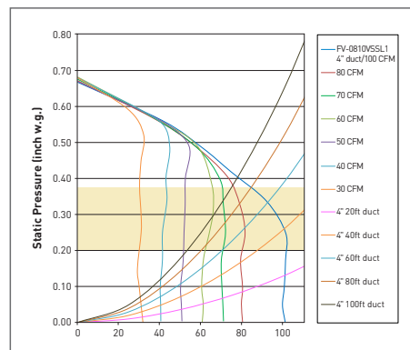
FV-0810VSSL1 80-100 CFM 4" Oval Duct
