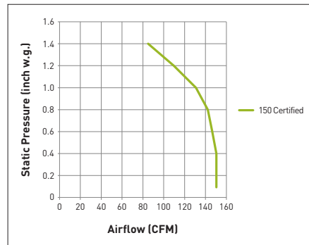
FV-15VE1T Net Supply
