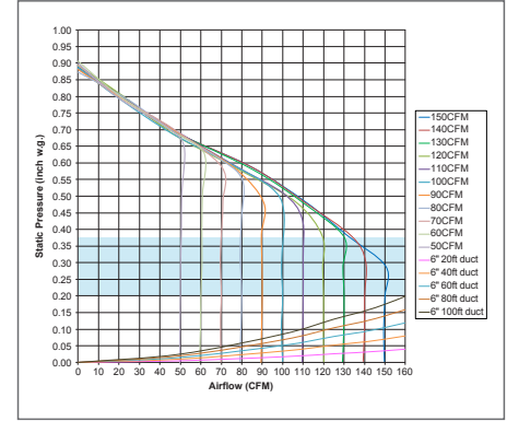
FV-15NLF51H 50-150 CFM 6" Duct
