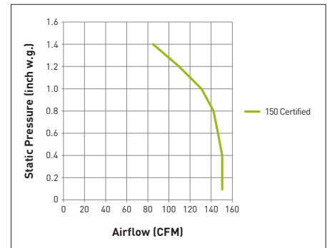
FV-15VE1S Net Supply
