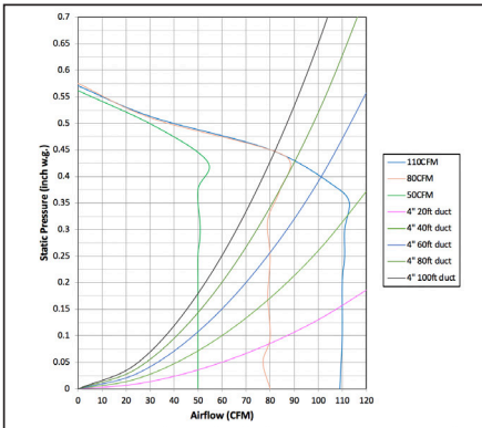
FV-0511VF1 - 4" Duct
