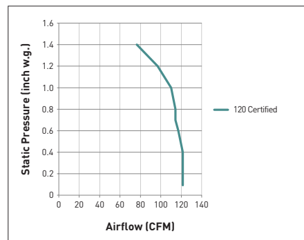
FV-12VE1T Net Supply
