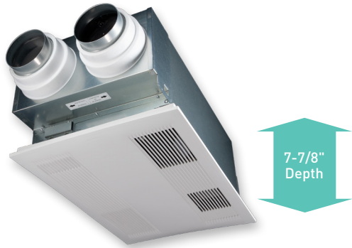
FV-06VE1 20-60 CFM
