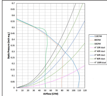
FV-0511VFC1 - 4" Duct
