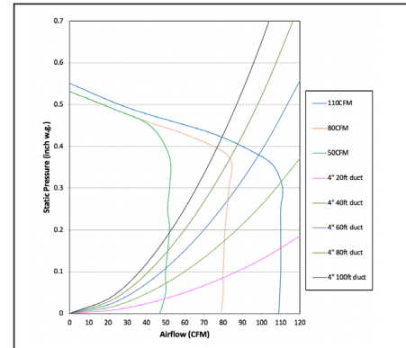
FV-0511VFL1 - 4" Duct
