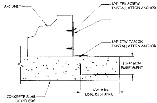
B 1 INSTALLATION DETAIL CONCRETE SUBSTRATE
