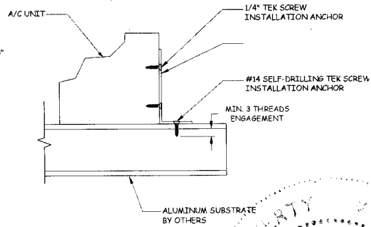
D 1 INSTALLATION DETAIL ALUMINUM SUBSTRATE
