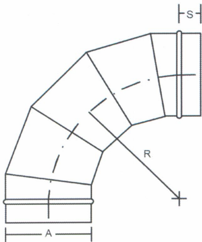
90° Elbow
