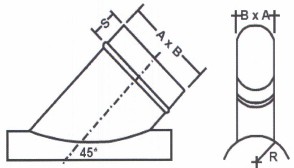
Oval Lateral Saddle Tap
